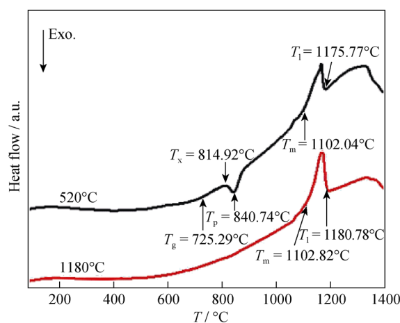
Fig. 4. DSC curves of the as-sintered FeSiBAlNi HEA prepared by SPS at different temperatures.
